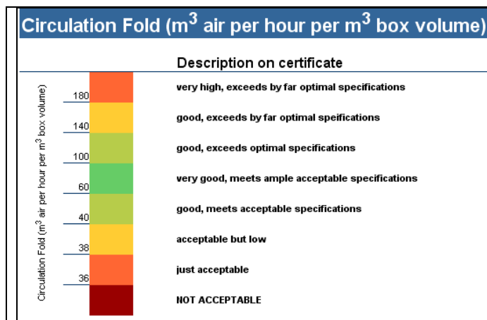
Figure 8: classification of air circulation capacity.
