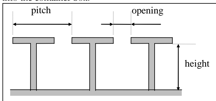
Figure 14: T-bar floors.
