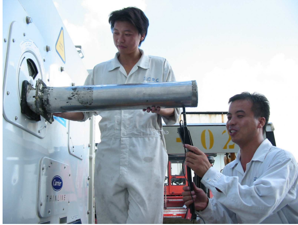
Figure 12: air speed measurement of fresh air outlet vent (step 4).
