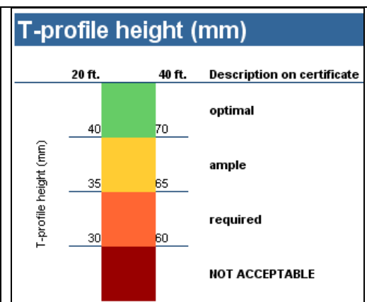
Figure 9: classification of T-bar height.
